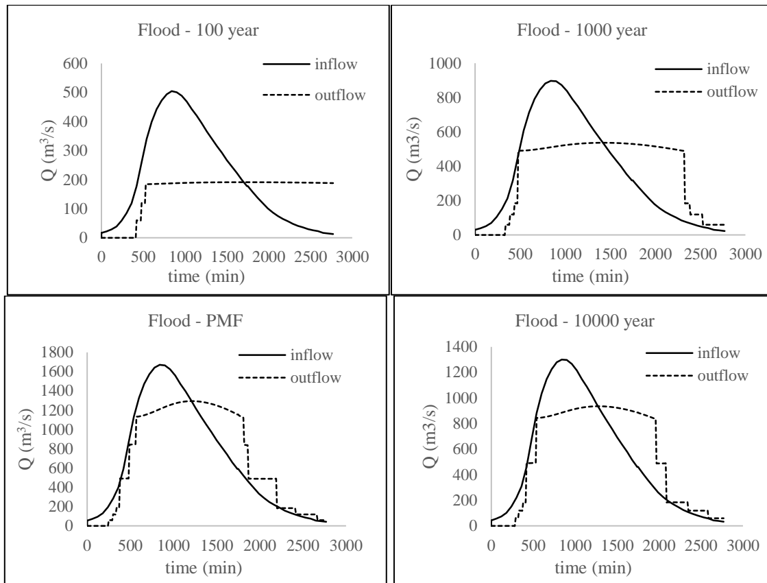
Fig. 8. inflow and outflow hydrograph for 100,1000,10000 and PWF floods
