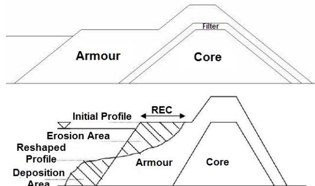
Fig. 1. Cross-section of berm breakwater two layer and three layer
