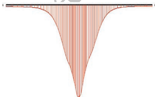
Vertical displacements (Uy) Extreme Uy -29.16*10 -3 m
