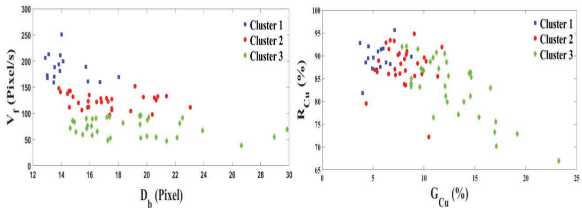
Figure 3. Clustering of froth images based on metallurgical parameters
