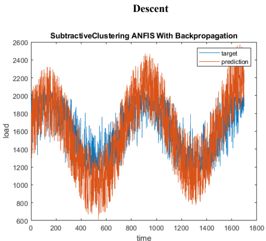
شکل ۱۴-ت: Subtractive clustering ANFIS with backpropagation
