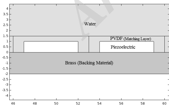
Fig. 5 Placement of Piezoelectric elements, medium, backing and matching materials in simulated linear phased array transducer
