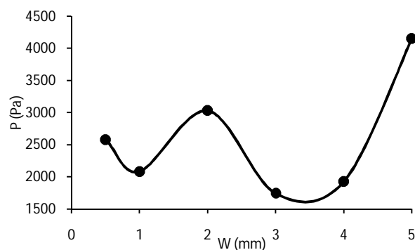
Fig. 16 Effect of width of piezoelectric elements on acoustic pressure of focal point
