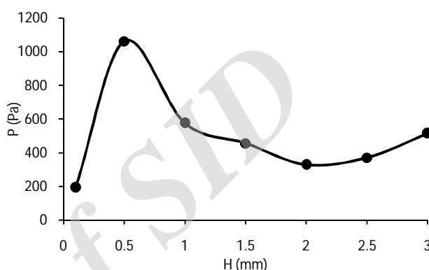
Fig. 15 Effect of thickness of piezoelectric elements on acoustic pressure of focal point
