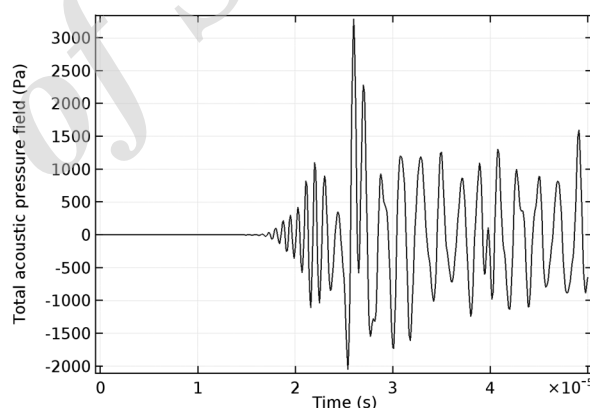
Fig. 11 Calculated acoustic Pressure in focal point ( 25 \text{ mm}, 0^\circ ) in term of time
