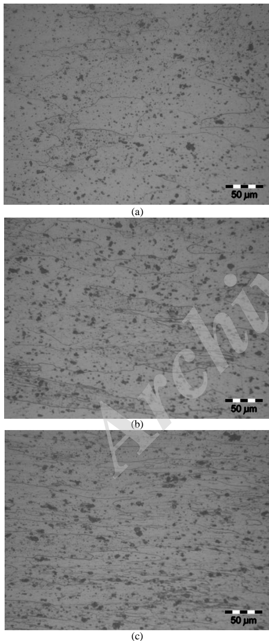
Fig. 4 Metallography images of T3 samples by: a) 15, b) 30 and c) 50 percent reduction in area
