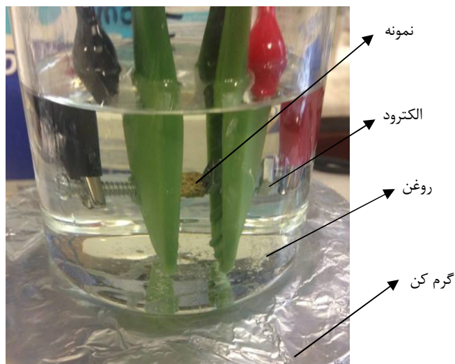
Fig. 5 Poling samples
