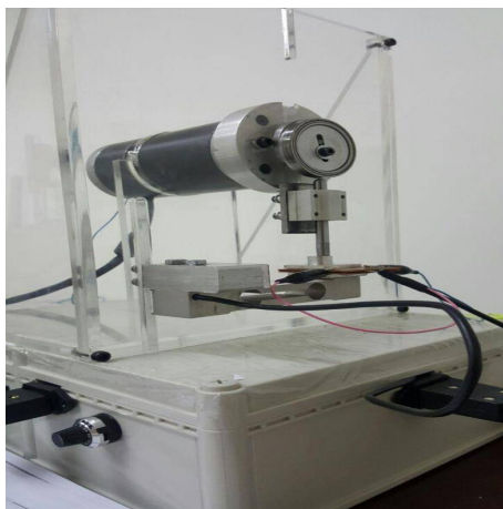
Fig. 6 Piezoelectric device
