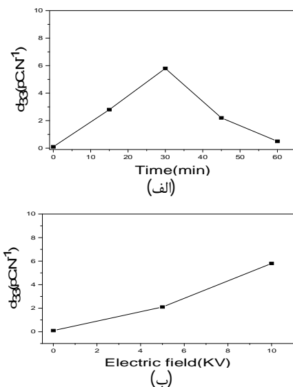
Fig. 11 Effects of polarization process on piezoelectric coefficient in group of scaffolds A: Polarization time B: Polarized electric field
