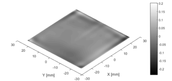
Fig. 12 Deviation between measurement and design surfaces after the fine localization process
