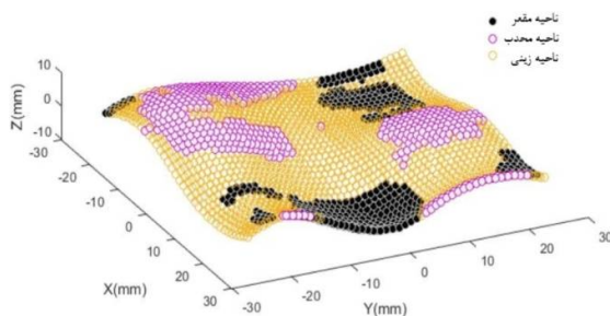
Fig. 4 Partitioned free-form surface
