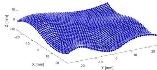
Fig. 3 Cloud points extracted from the free-form surface
