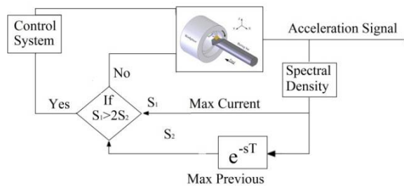
Fig. 16 Block diagram of close loop controller with time delay
