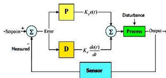
Fig. 17 Block diagram of PD controller
