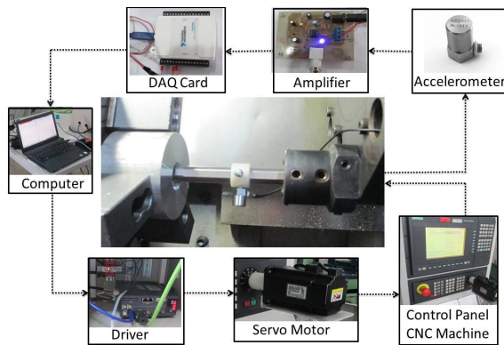
Fig. 25 Hardware architecture of experimental setup
