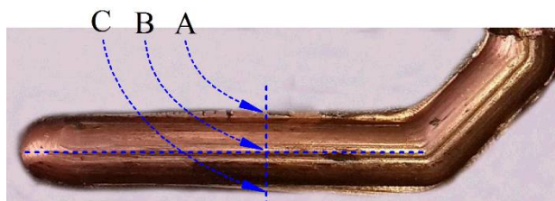
Fig. 9 Picture of a copper sample for measurement of hardness changes after 4th pass
