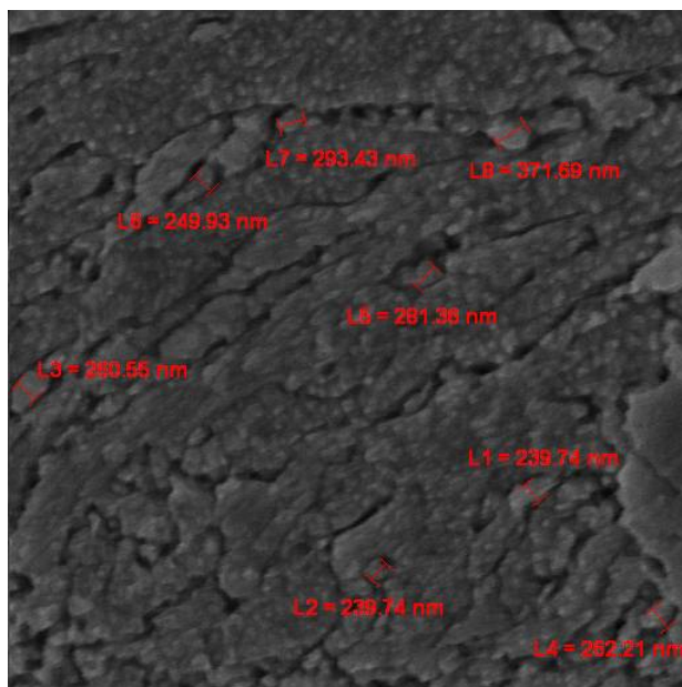
SEM MAG: 20.00 kx Det: SE Detector VEGA TESCAN SEM HV: 15.00 kV WD: 7.9451 mm 2 μm (الف) RAZI Date(m/d/y): 06/30/08 Vac: HiVac
