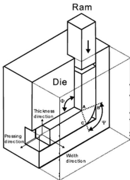
Fig. 1 Schematic view of Equal Channel Angular Pressing Extrusion
