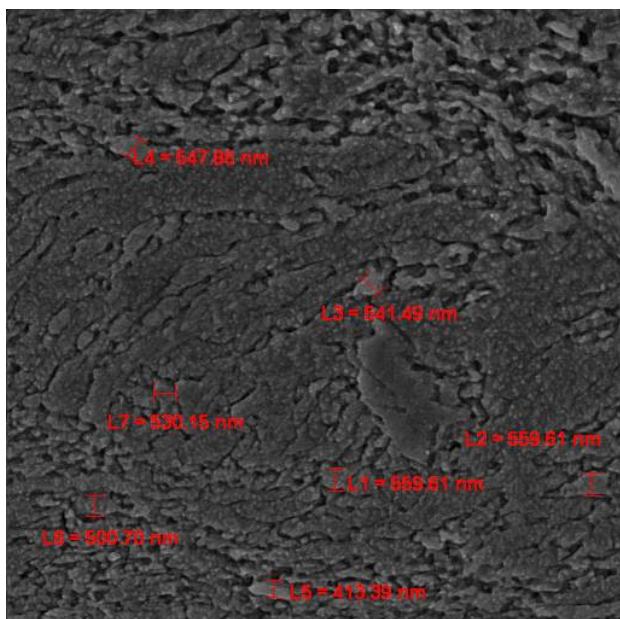
Fig. 7 SEM image from microstructure of ECAPed copper after 4 th pass extrusion in 90° internal die channel
