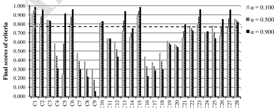
Fig. 5. Final scores of initial criteria in DMs' viewpoints
