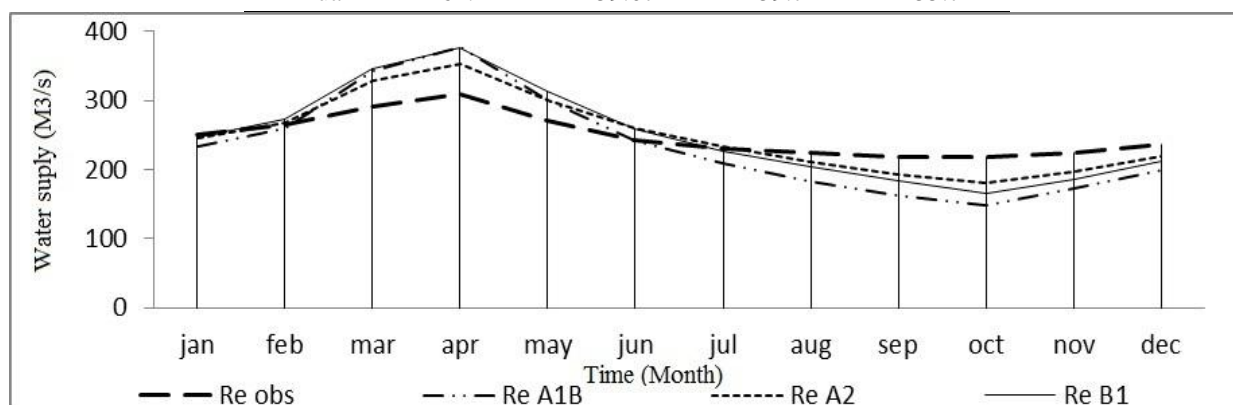
Fig. 9- Operation rule curve for the dam in the base and future period
