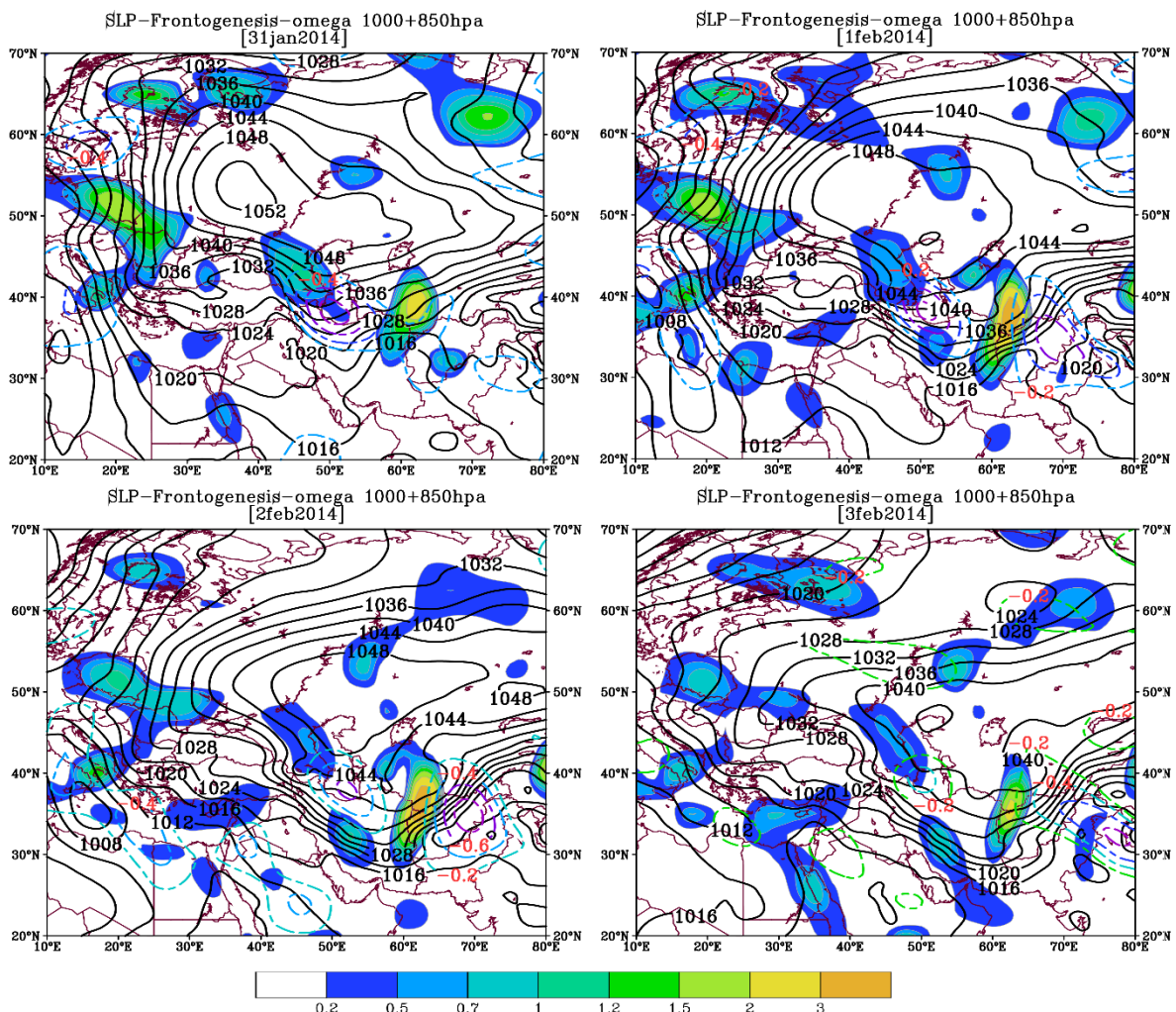
Fig. 2- Condition of pressure patterns, frontogenesis and vertical velocity in January 31 to February 3
