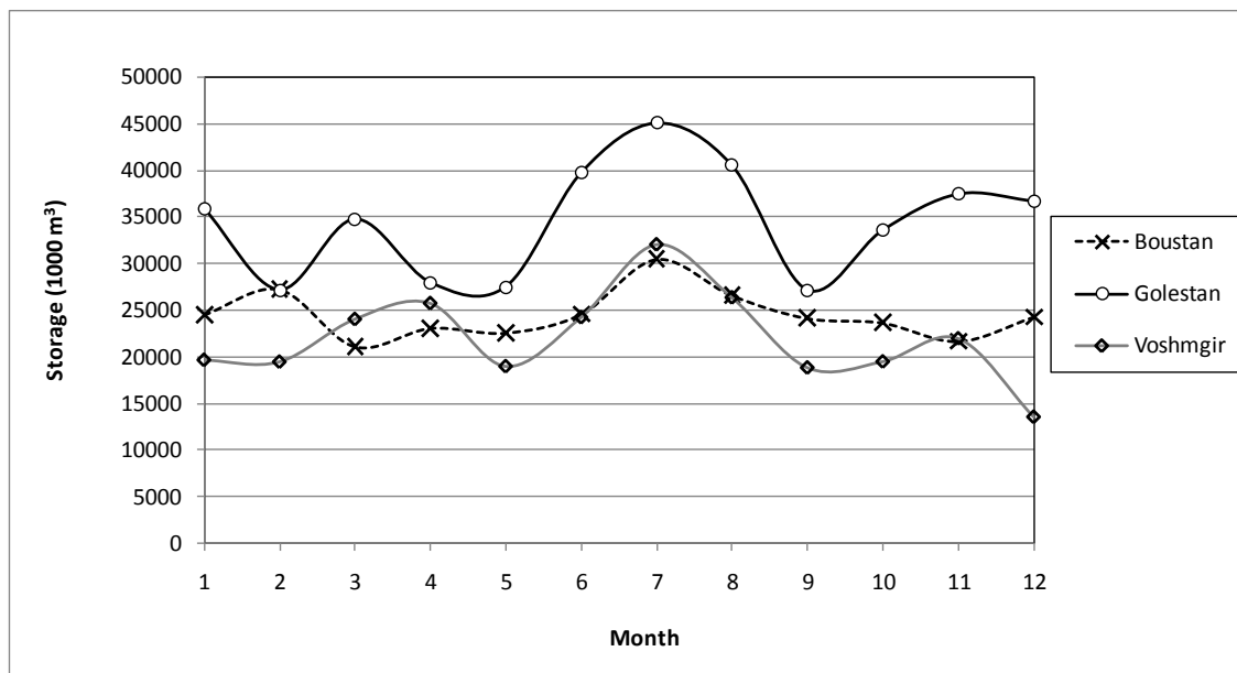
Fig. 19- Average annual optimum storages of dam reservoirs in the Gorganroud basin
