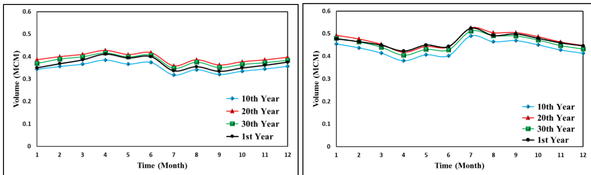
Fig. 14- Discharge for Scenario 3: (a) from the lake to the aquifer, and (b) from the aquifer to the lake
