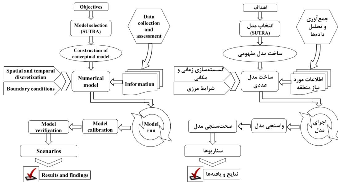
Fig. 4- Groundwater modeling steps for Ajabshir plain
