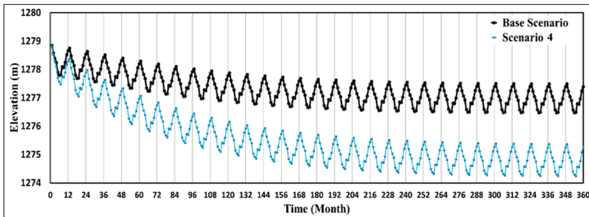
Fig. 15- Groundwater hydrograph of Ajabshir aquifer over 30-years period for scenario 4
