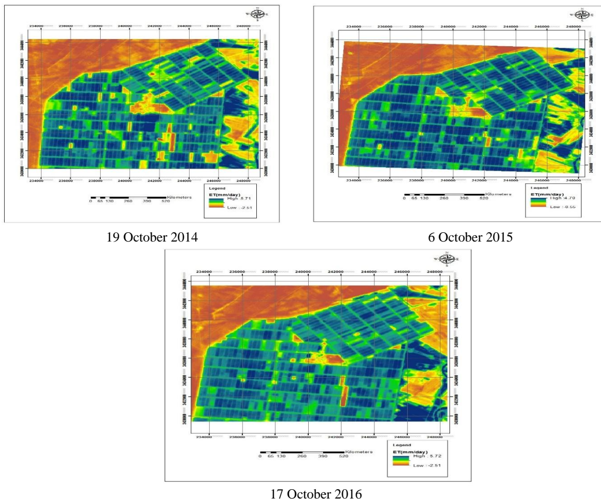
Fig. 3- The maps of actual evapotranspiration from Landsat 8 and MODIS fusion images and SEBAL algorithms
