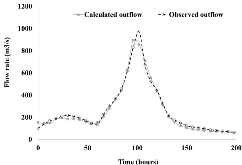
Fig. 3- Comparison of the measured and calculated hydrographs obtained with the proposed NL6 model (second case study)
