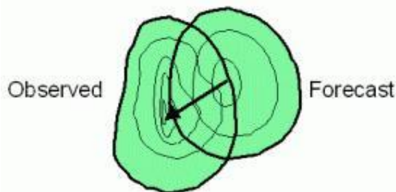
Fig. 2- Schematic of the prediction and observation rain areas in the CRA method
