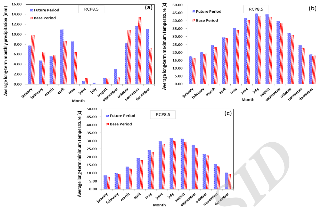
Fig. 3- Comparison of the long-term average monthly (a) rainfall, (b) maximum temperature, and (c) minimum temperature for the base period (2005-1986) and the upcoming period (2039-2020) under RCP8.5 scenario
