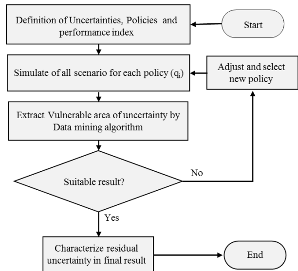
Fig. 2- RDM Flowchart
