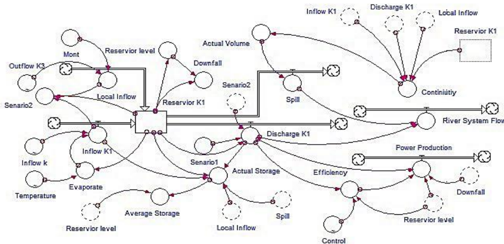
Fig. 2- The structure of Production model for hydropower system
