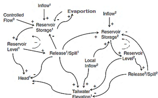
Fig. 1- Causal loop diagram for a reservoir hydropower system (Teegavarapu & Simonovic, 2014)
