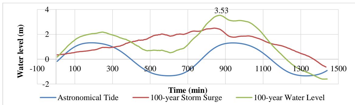
Fig. 5- A 100-year Water level Time Series
