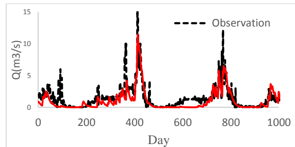
Fig. 5- Comparison of observed and simulated flow for the calibration period
