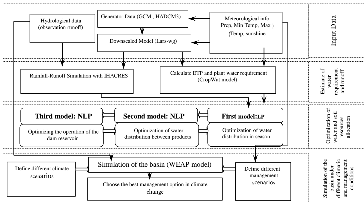
Fig. 1- Research Flowchart
