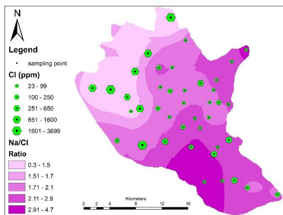
Fig. 8- Spatial distribution of the Na^+/Cl^- ratio and Cl^- concentrations
