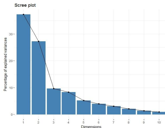
Fig. 2- Investigated components in extracted Scree plot
