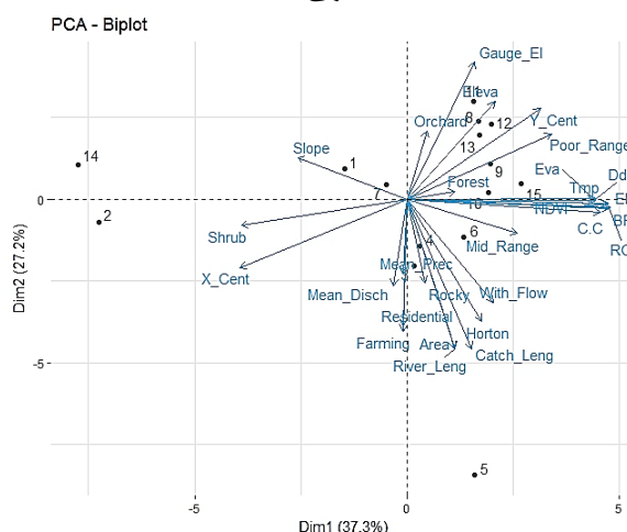
Fig. 3- Biplot of principle components
