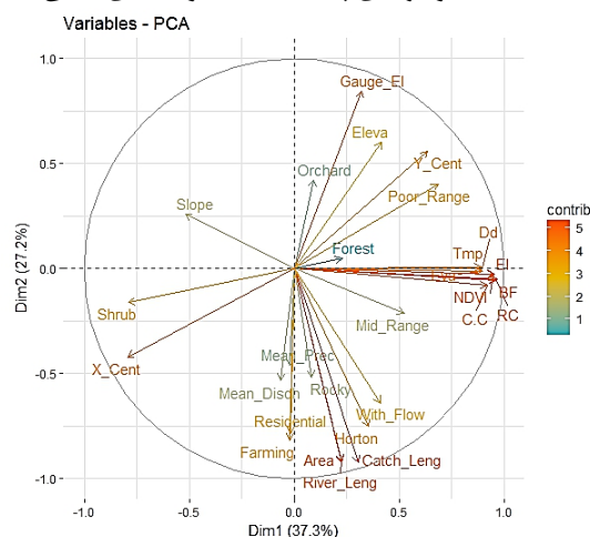
Fig. 4- Biplot graphs of Dim 1 & 2 using PCA algorithm
