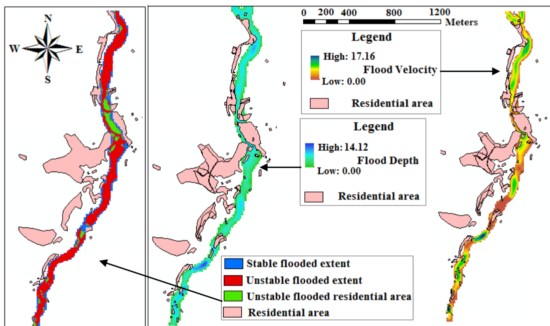
Fig. 4- 500-year flood depth and velocity extent as well as unstable flooded residential areas in Soleghan
