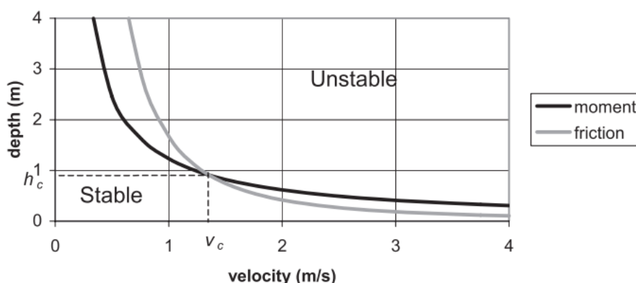
Fig. 2- Theoretical boundaries for moment and friction instability (after Jonkman and Penning-Rowse, 2008)
