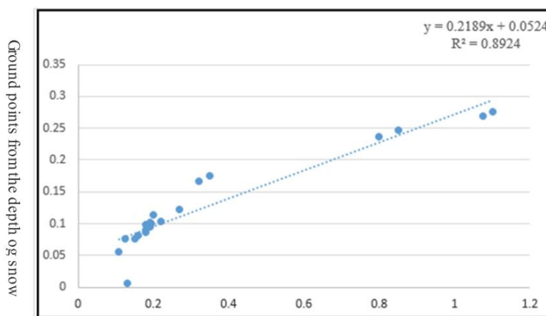
Estimated snow depth points from the D-InSAR technique
