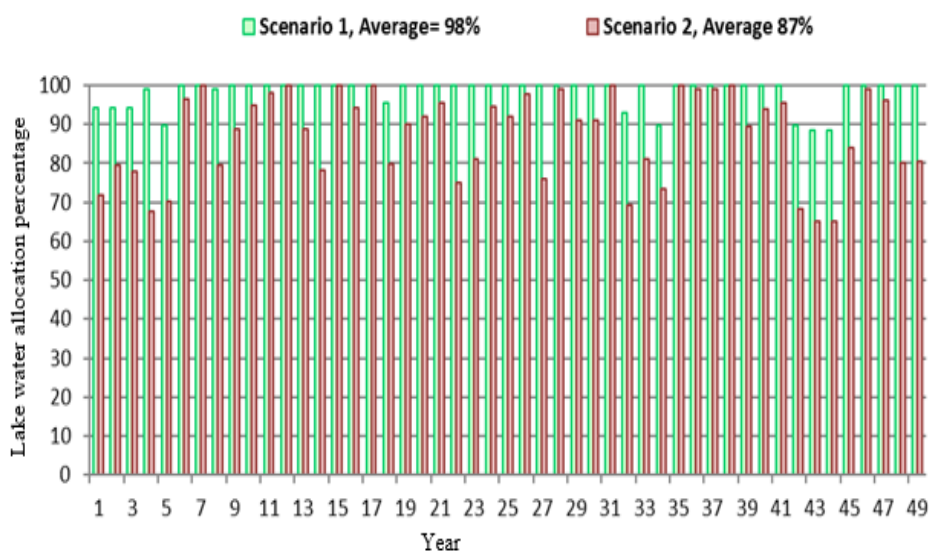
Fig. 12- The amount of water allocation to the Lake for East Azerbaijan province under LU drought plan by Scenario 1 (full allocation of LU water requirement) and scenario 2 (partial allocation of LU water requirement)
