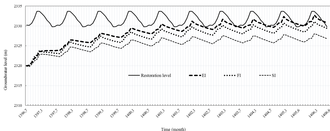
Fig. 6- Namdan aquifer groundwater level changes on the basis of three indicators, stability, filling and restoration for the ten-year simulation period
