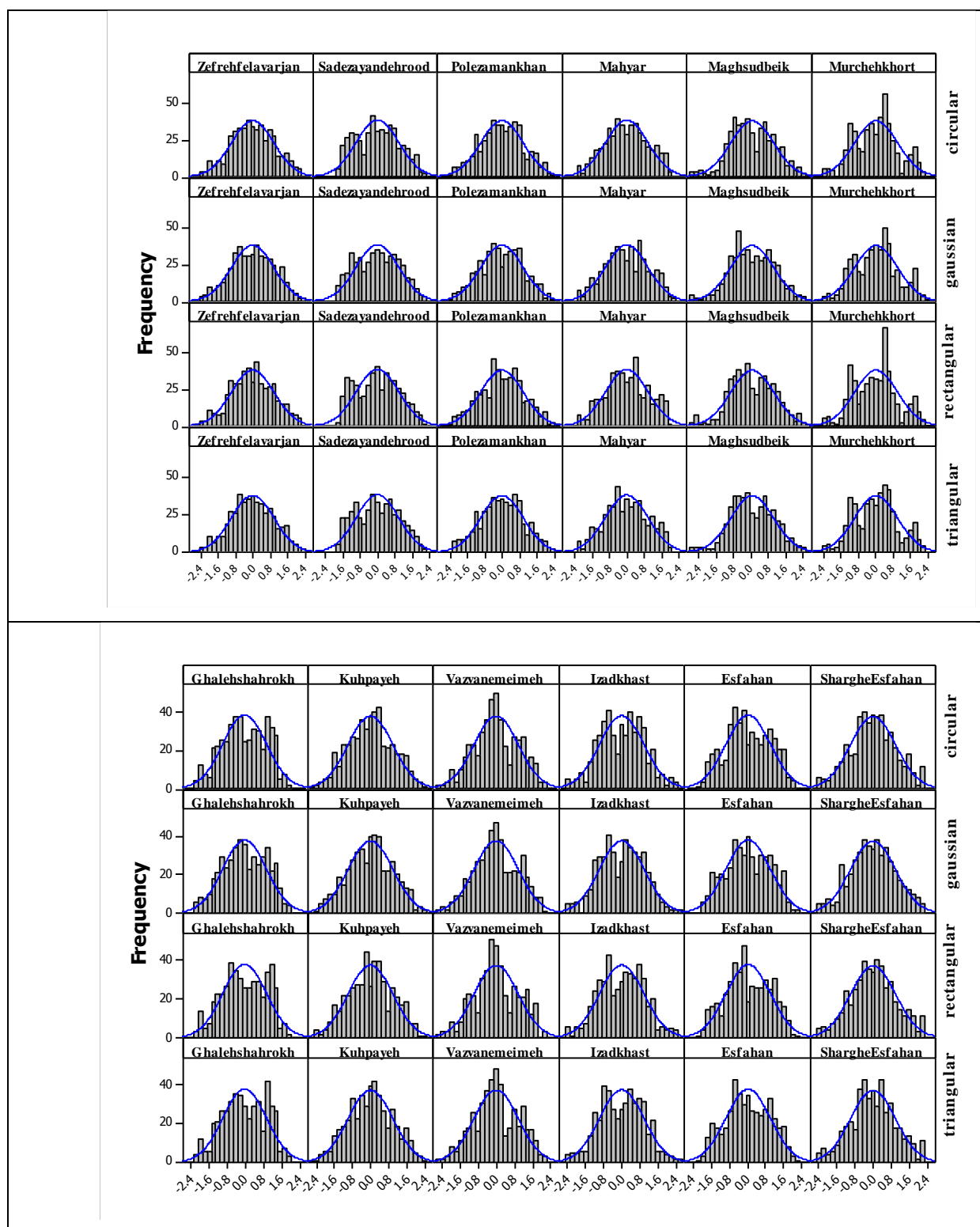
Fig. 3- Frequency histogram of SPEI in all staisn
