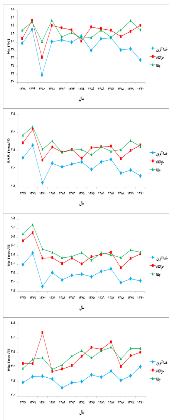
Fig. 2- a) Time variations of \text{Na}^+ , SAR and \text{Mg}^{2+} parameters at Khodaafarin, Khazangah and Julfa Stations
