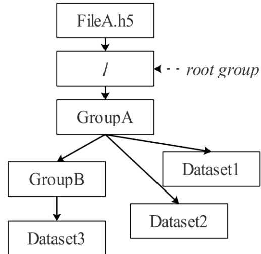
Fig. 2- An HDF5 file with hierarchical structure (National Center for Supercomputing Applications, 2016)
