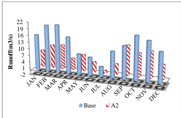
Fig. 6- Long-term variations of the runoff simulated by the model in the upcoming period relative to the base period
