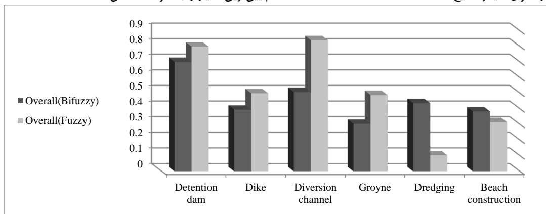
Fig. 2- Overall ranking based on Fuzzy and Bifuzzy methods
