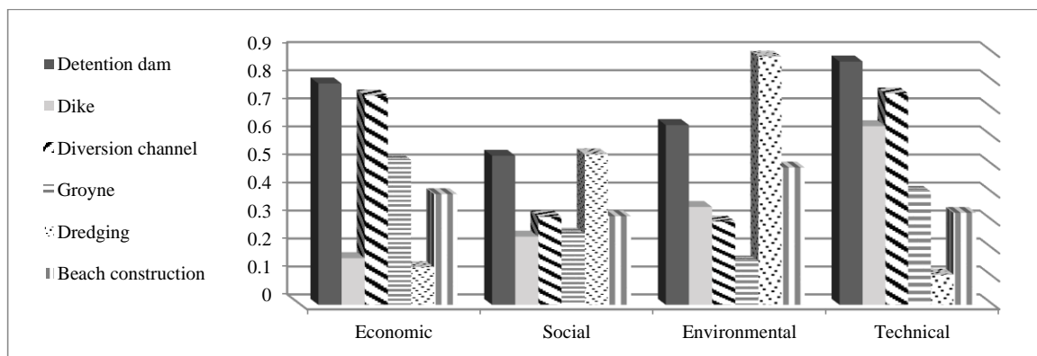
Fig. 3- Ranking of projects according to different criteria
