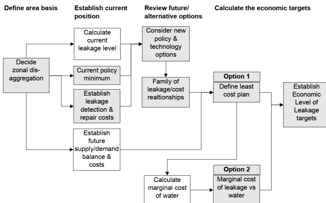
Fig. 2- Leakage target setting guideline with respect to economic, social and environmental costs ( Tripartite Group, 2002)
