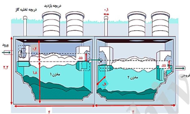
Fig. 2. Dimensions (in m) of the septic tank used in the Times project
