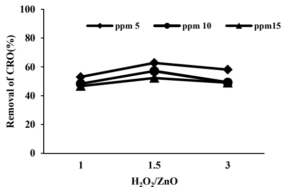
Fig. 2. Effect of H_2O_2/ZnO molar ratio on Ceftriaxone removal efficiency
