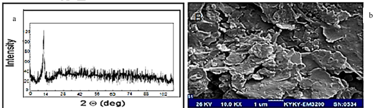
Fig. 1. a) XRD pattern of GO, B) SEM image of GO
