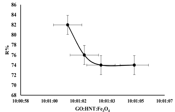
Fig. 10. Effect of composition ratios on zinc removal by M-HNT/GO adsorbent
