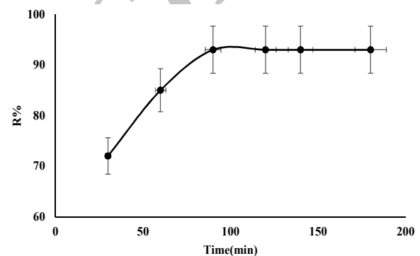
Fig. 11. Effect of contact time on zinc removal by M-HNT/GO adsorbent
