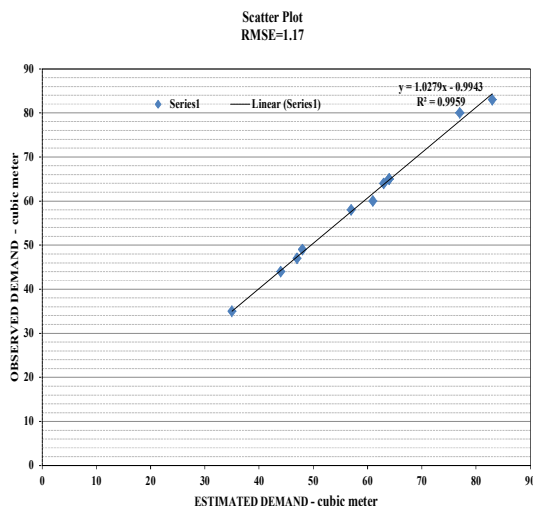
Fig. 13. Scatter plot for Geostatistical model
