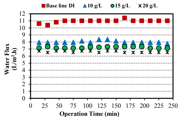
Fig. 2. The effect of salt concentration in simulated PW samples (0 to 20 g/L) as the feed solution on water flux (in absence of oil and with sodium chloride 1.2 M as the draw solution at 25 °C)
