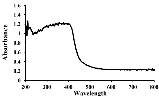
Fig. 3. DRS pattern of Bi 2 O 3 nanoparticles calcined in 600 °C
