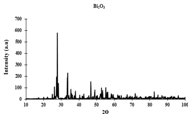
Fig. 1. XRD pattern of Bi 2 O 3 nanoparticles calcined in 600 °C
