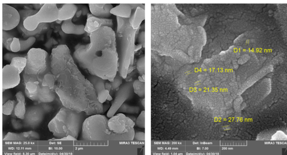
Fig. 2. SEM image of Bi 2 O 3 nanoparticles calcined in 600 °C
