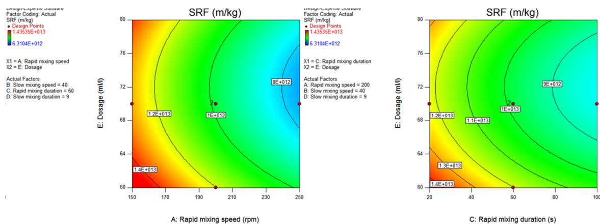
Fig. 9. Effect of mixing speed and duration in rapid rotating on SRF contour plot
