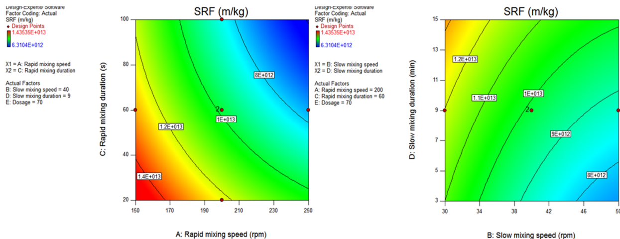
Fig. 7. Effect of mixing speed and duration on CST contour plot
