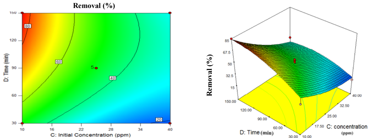
Fig. 8. Contour and 3D plots for Hg(II) removal vs. Contact time and Initial concentration
