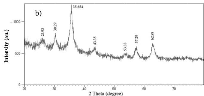
Fig. 2. XRD patterns of (a) MWCNT (b) Magnetic MWCNT (b)
