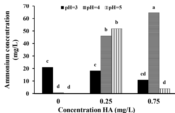
Fig. 5. Interaction of humic acid and pH on the concentration of ammonium nitrate removal process of water containing 30 mg/L of nitrates
