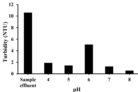
Fig. 1. Effect of different pH on the turbidity omission using constant concentration of PAC in Qom wastewater treatment plant
