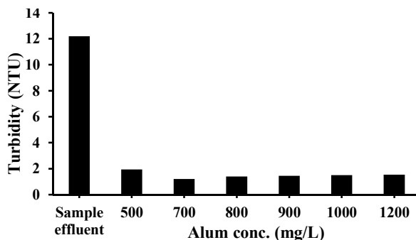
Fig. 2. Effect of different concentrations of alum in pH = 8, in the amount of turbidity reduction in Qom wastewater treatment plant
