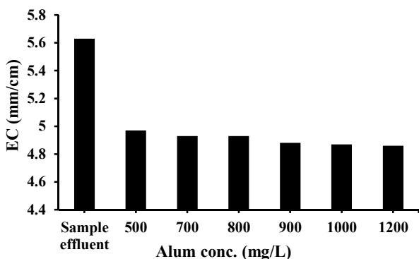
Fig. 5. Effect of different alum concentration at pH=8, in the amount of EC change in Qom wastewater treatment plant
