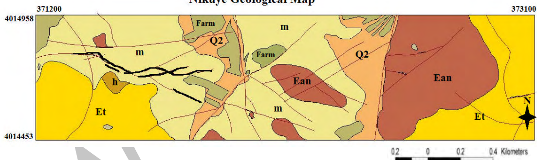
Nikuye Geological Map
