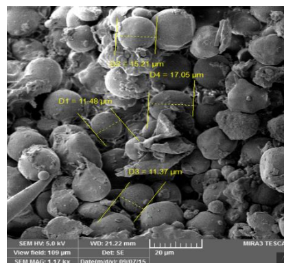
Figure2- Steam flaked sorghum grain
