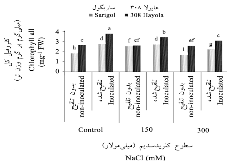
Figure 6. Mean of total chlorophyll of canola cultivars under salinity stress and inoculation with P. fluorescens FY3.
