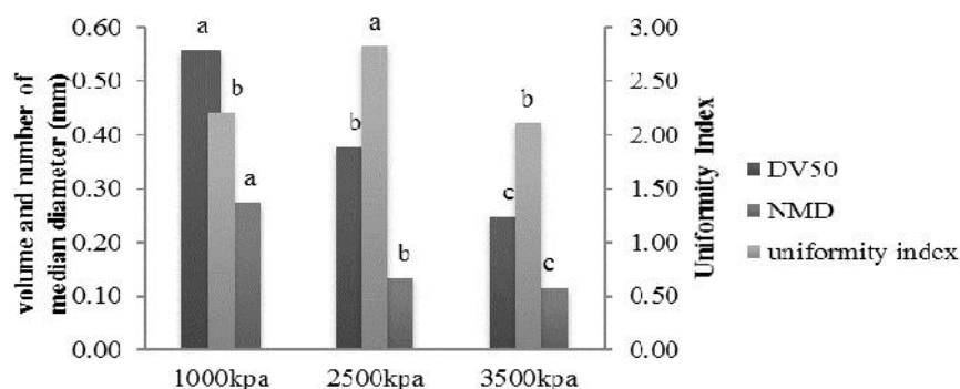
Fig. 3. Mean comparison of the effect of the pressure on the volume median diameter (50%), number median diameter and spray quality index
